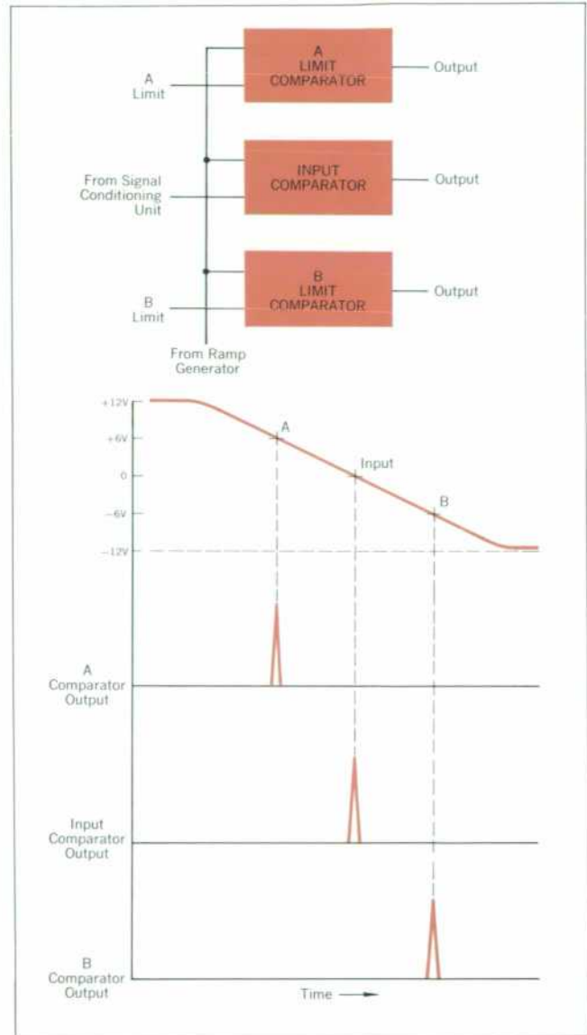
Fig. 4. Time sequence of the comparators. In this example, the A limit voltage has been set to +6 volts, the B limit voltage is -6 volts and the input voltage is 0 volts. When the ramp voltage, reaches +6, 0 and -6 volts in that order, the A limit comparator, input comparator and B limit comparator generate trigger pulses in the same sequence as shown.
